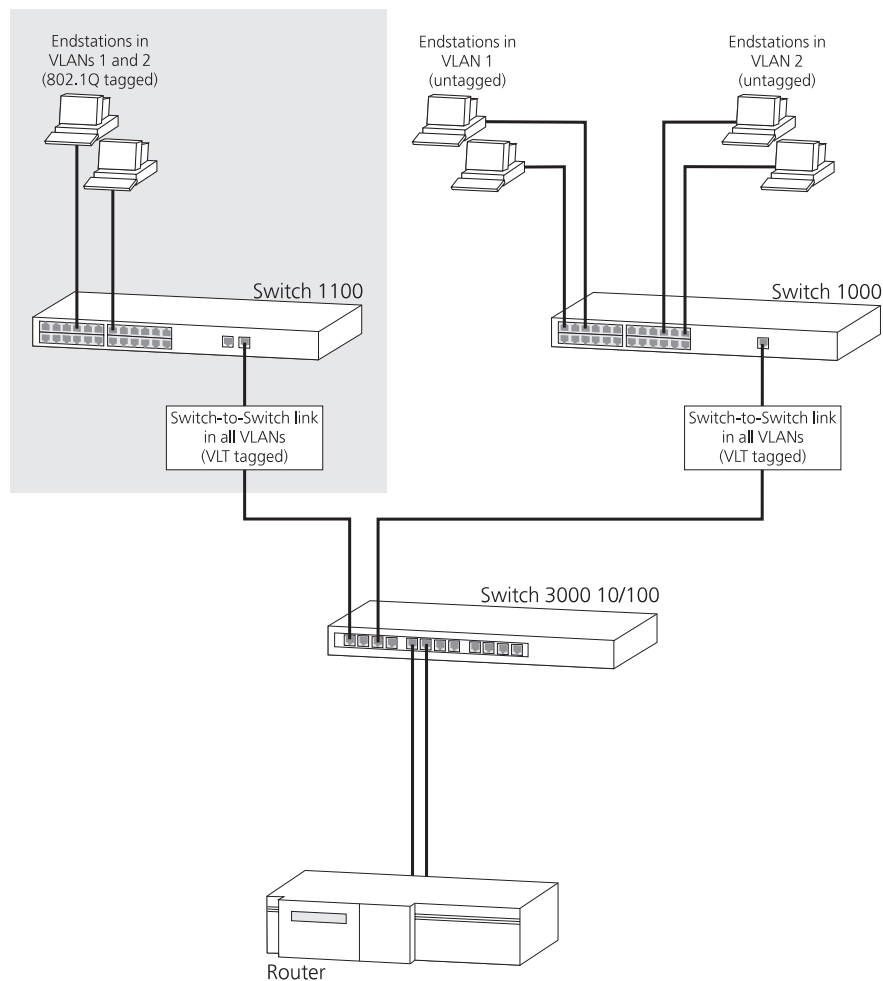
Figure 37 Connecting to legacy VLANs using VLTs
