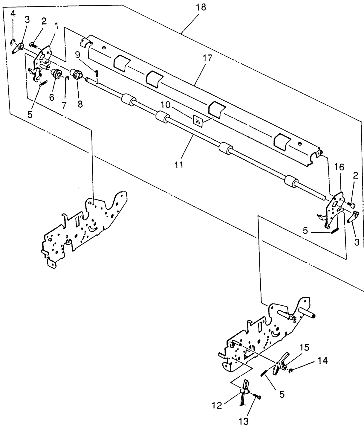
FIGURA 9-13 Espulsione Carta (923) FIGURE 9-13 Paper Eject (923)
