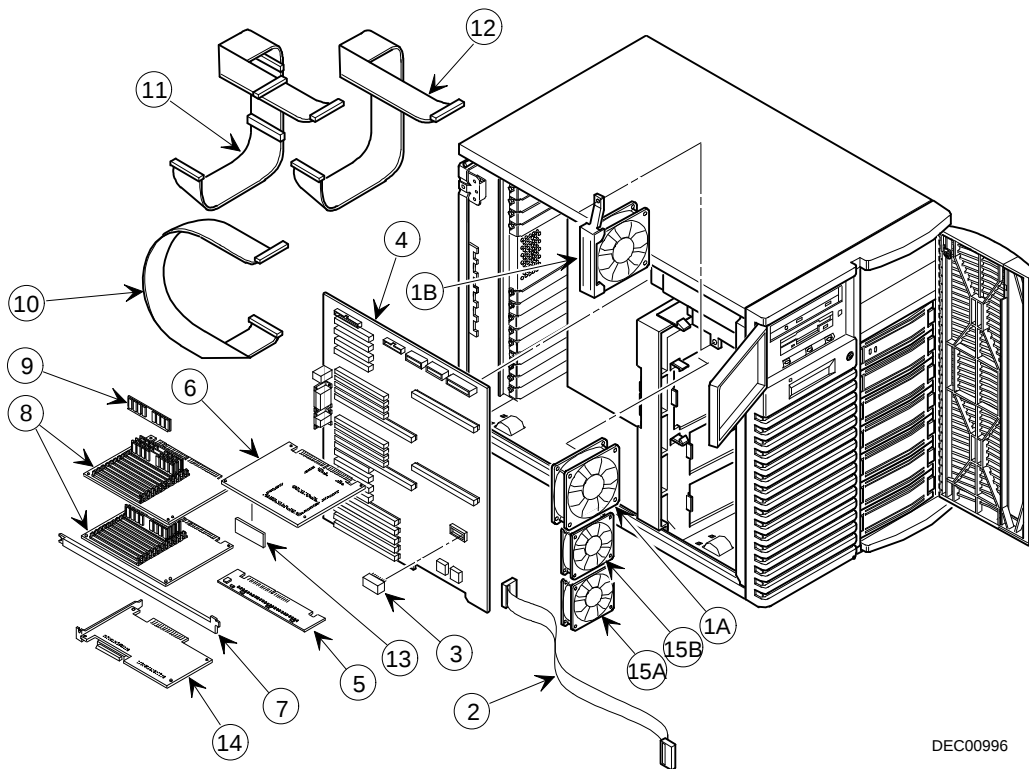
Server Left-Side View
