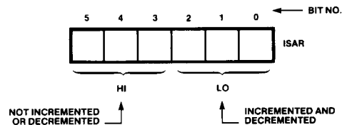
Figure 2 F8 Programming Model
