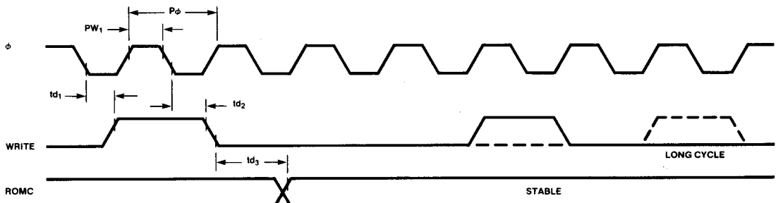
Figure 8 ROMC Timing Signals Output by F3850 CPU
