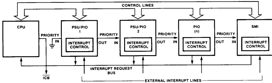
Figure 13 F8 System Interrupt Interconnection
