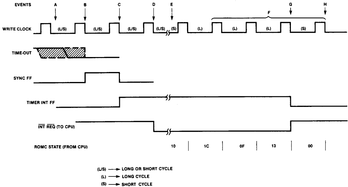
Figure 16 External Interrupt Sequence
