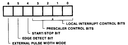
Figure 11 F3856 ICR Configuration
