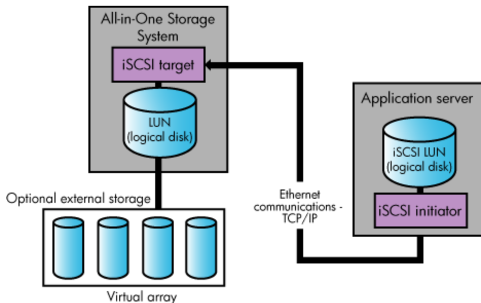
Figure 6 Application storage infrastructure
