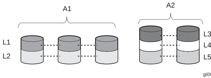
Figure 5 Two arrays (A1, A2) and five logical drives (L1 through L5) spread over five physical drives
