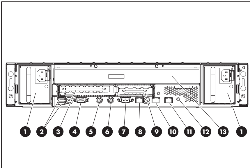
Figure 14 HP StorageWorks 1200 All-in-One Storage System rear panel
