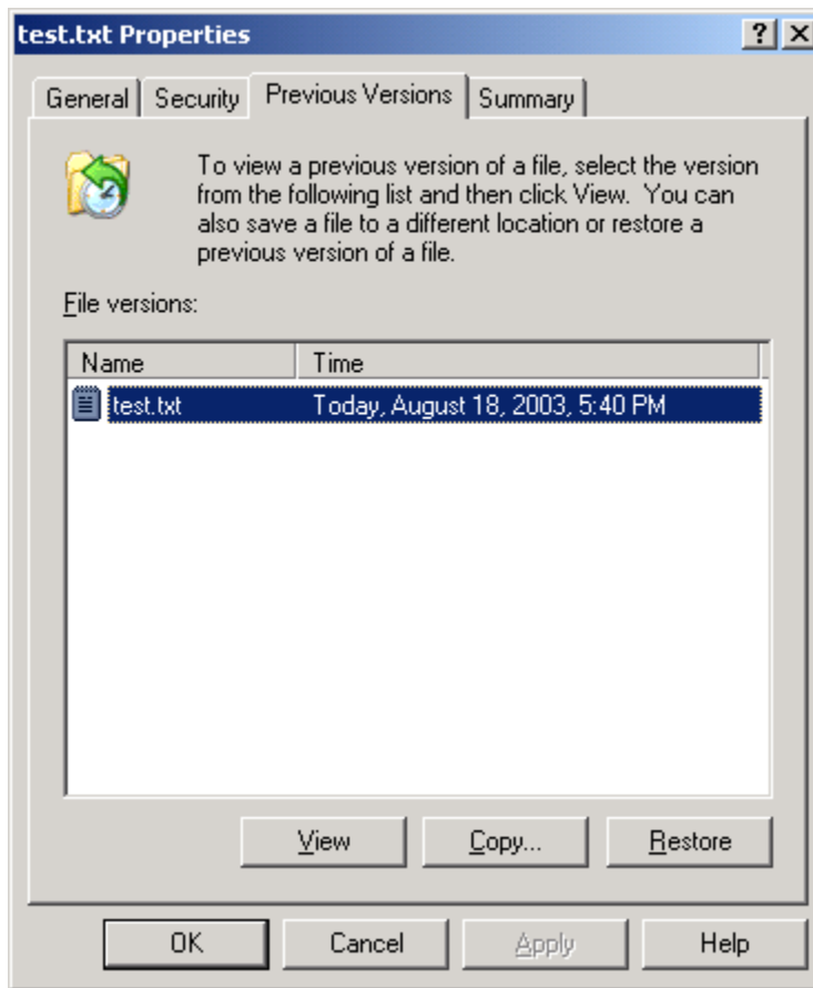
Figure 19 Client GUI
