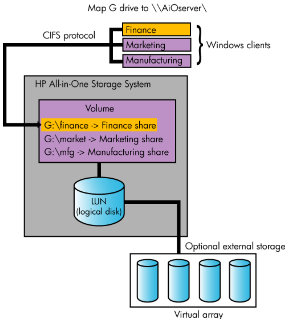
Figure 7 Shared folder storage infrastructure
