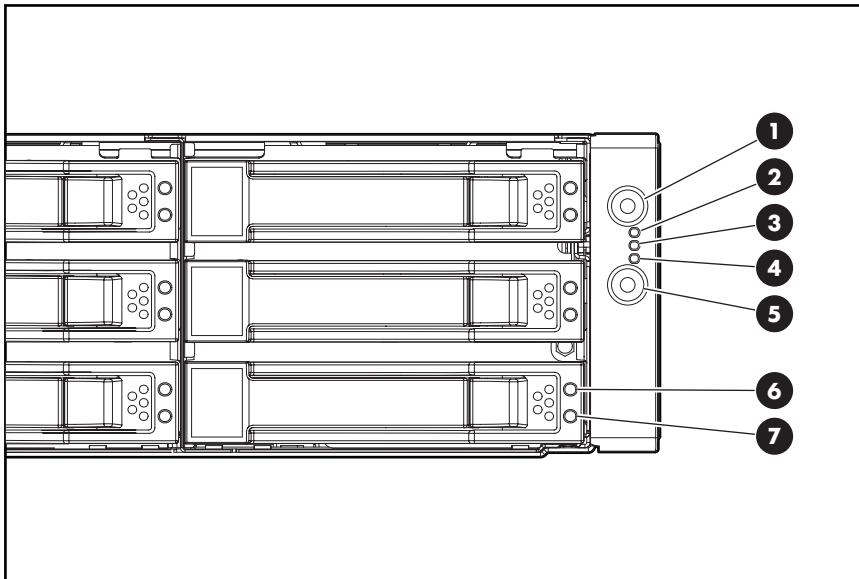
Figure 13 HP StorageWorks 1200 All-in-One Storage System front panel
