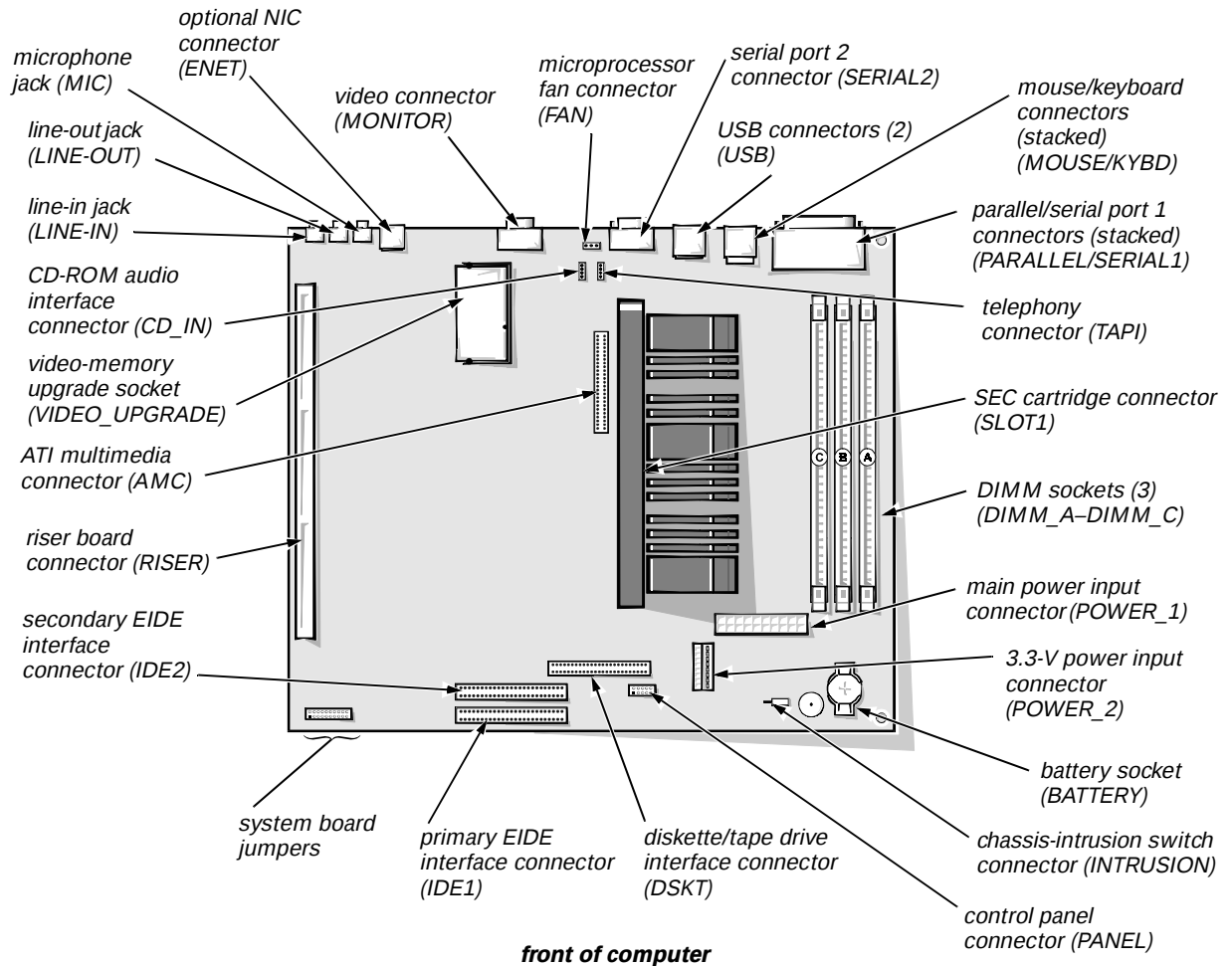
Figure 5-18. System Board Components
