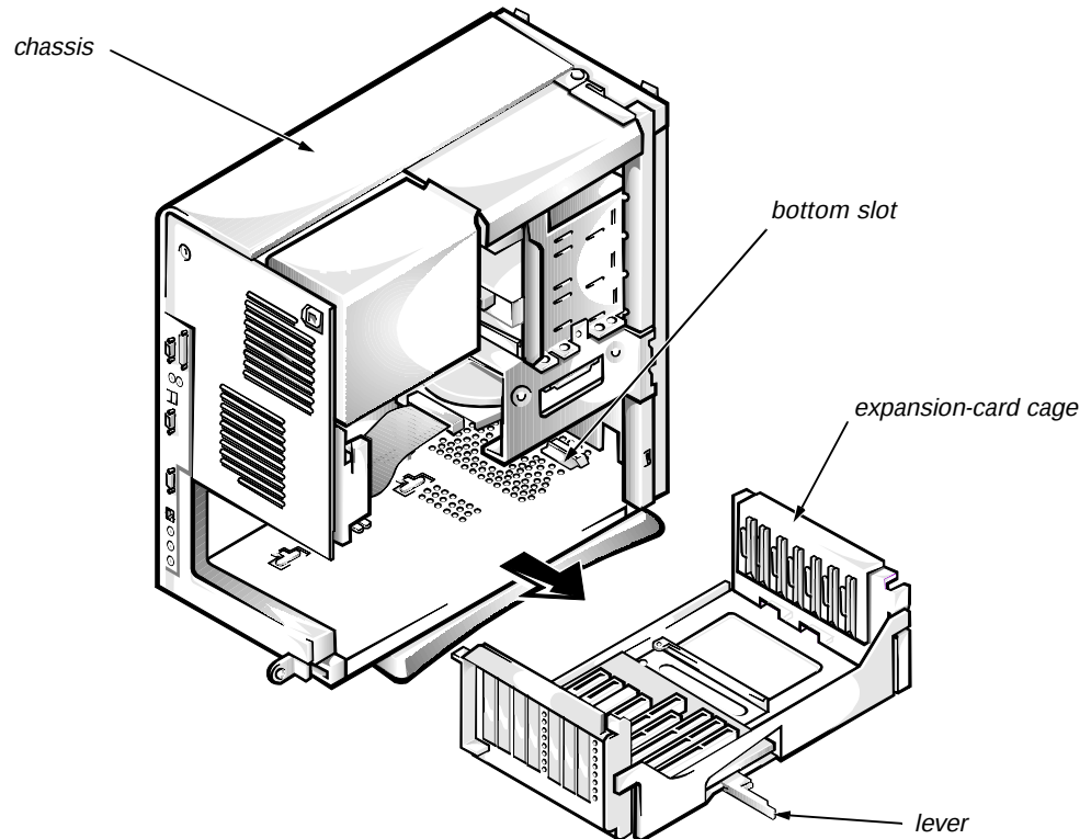
Figure 6-16. Expansion-Card Cage Removal
