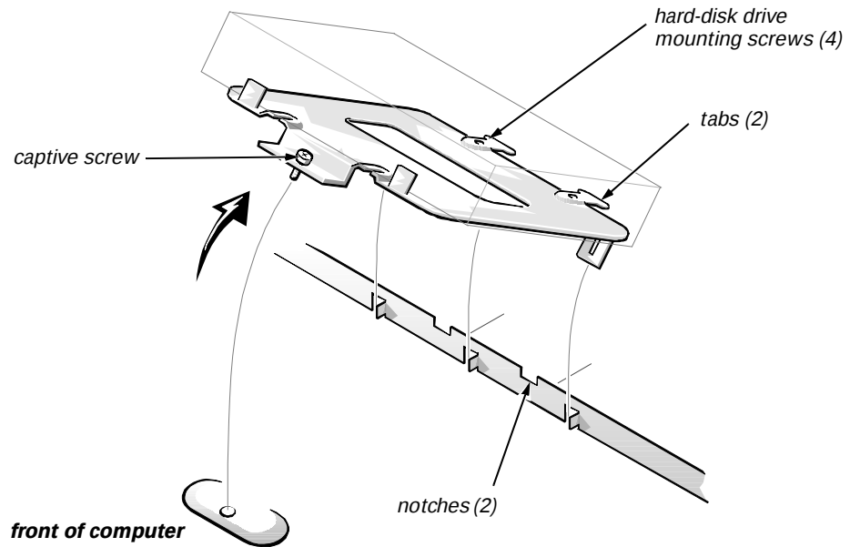
Figure 4-9. Hard-Disk Drive Assembly Removal
