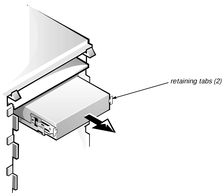
Figure 6-11. 5.25-Inch Drive Assembly Removal
