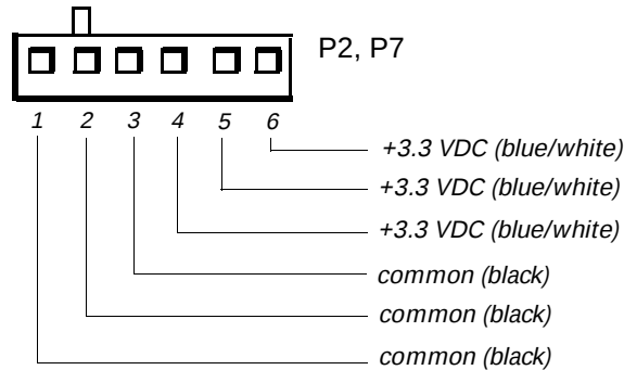
Figure 1-17. DC Power Connectors P2 (Low-Profile Chassis) and P7 (All OptiPlex GX1 Chassis)
