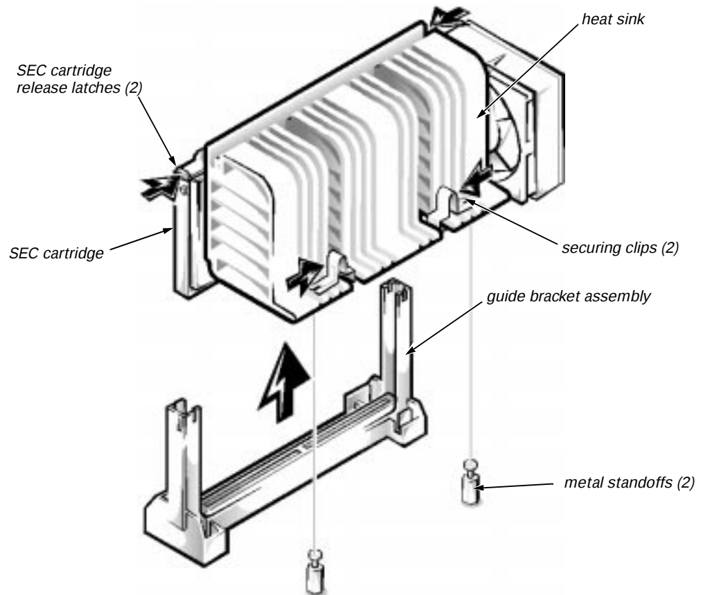
Figure 4-19. SEC Cartridge/Heat Sink Removal
