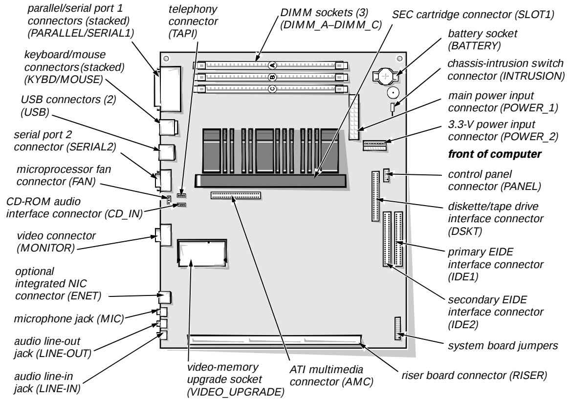
Figure 6-20. System Board Components
