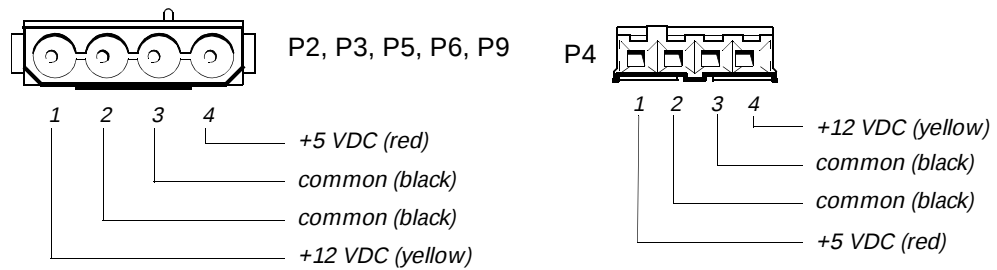
Figure 1-16. DC Power Connectors P2 (Midsize and Mini Tower Chassis); P3, P4, P5, P6, and P9 (All OptiPlex GX1 Chassis)
