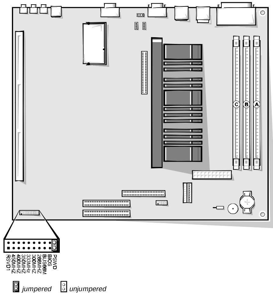
Figure 1-13. System Board Jumpers
