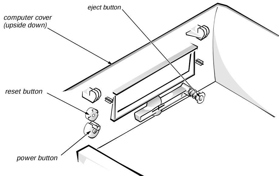
Figure 4-3. Eject, Power, and Reset Button Removal
