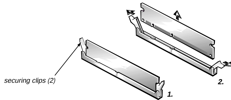
Figure 6-21. DIMM Removal
