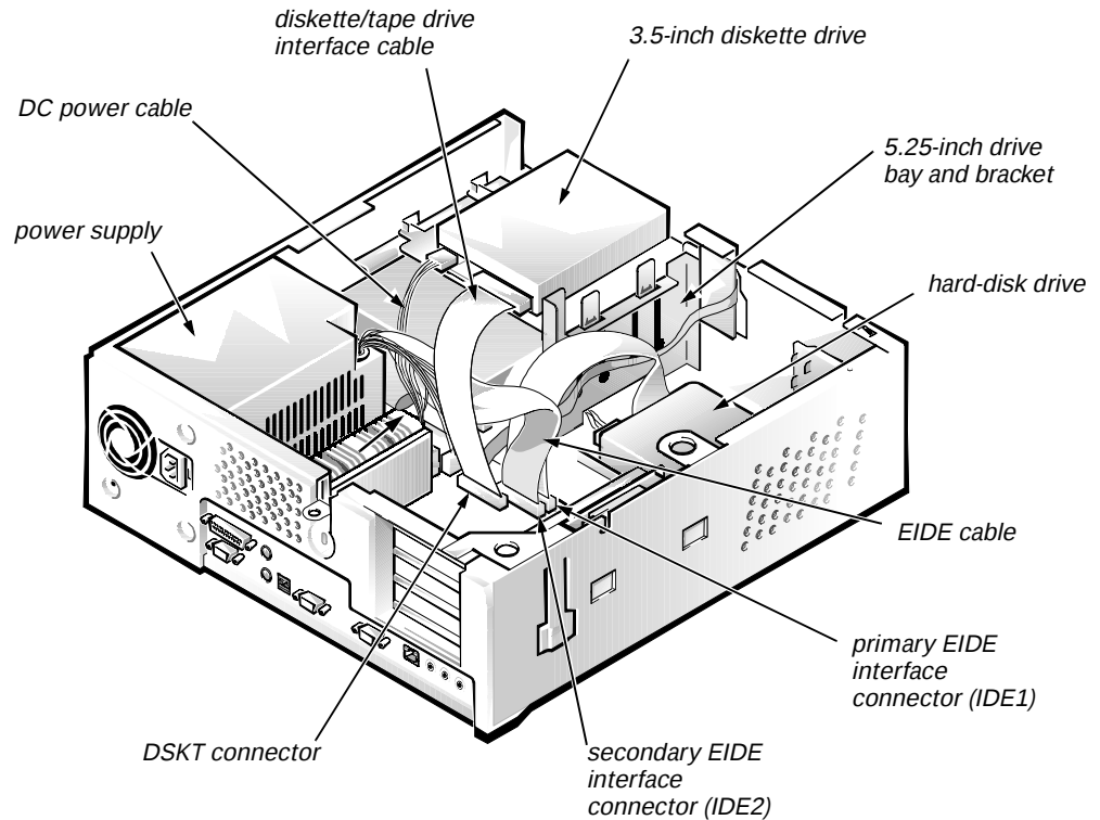
Figure 4-6. Drive Hardware
