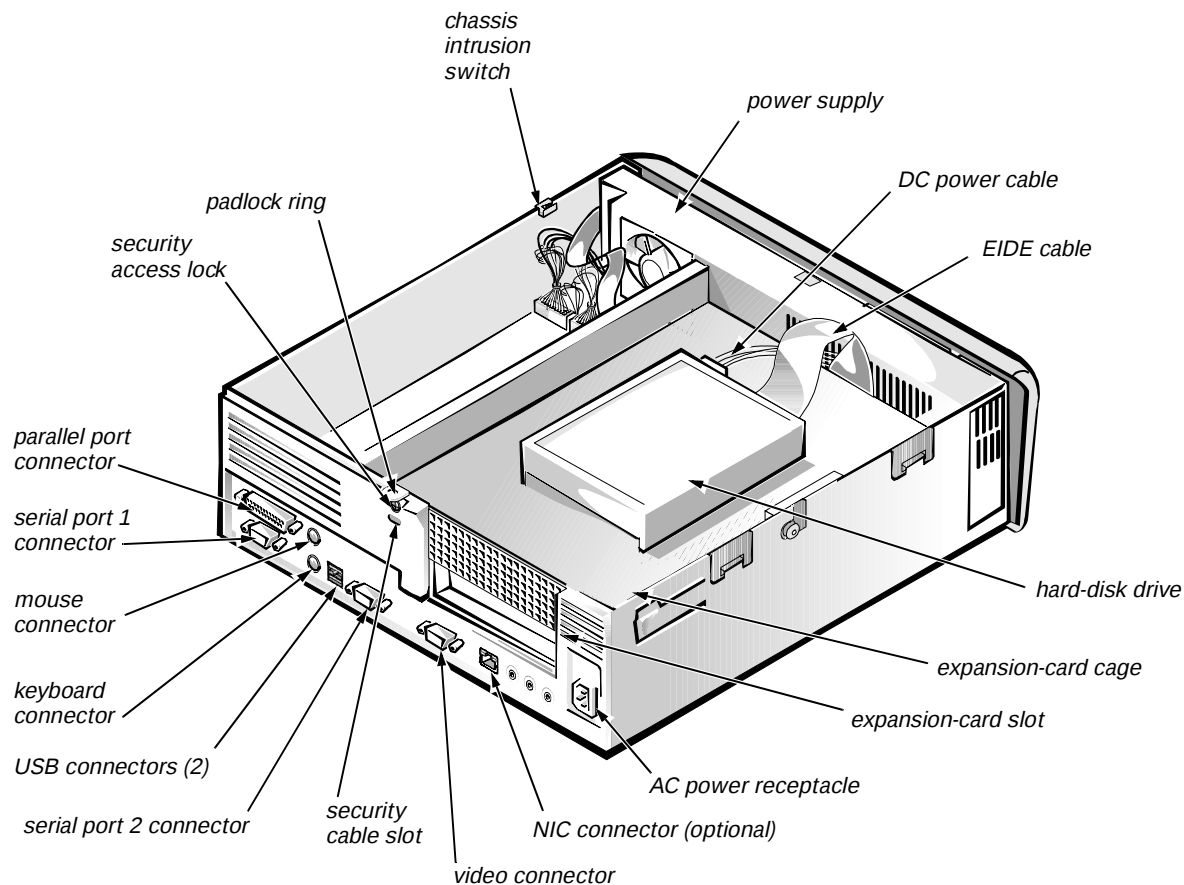
Figure 1-6. Internal View of the OptiPlex NX1 Chassis
