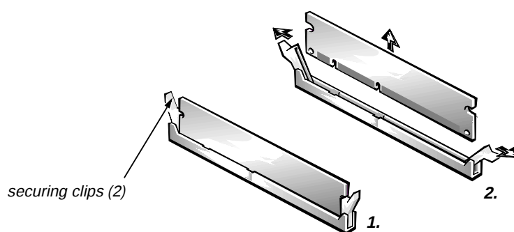
Figure 5-19. DIMM Removal
