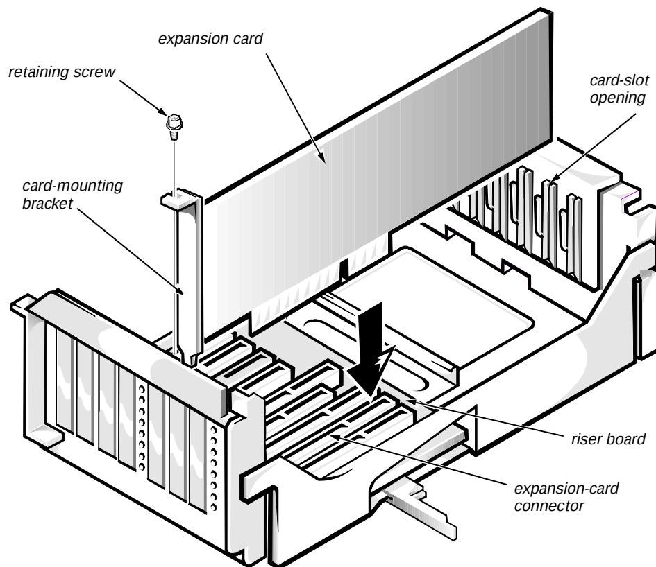
Figure 6-17. Expansion-Card Removal
