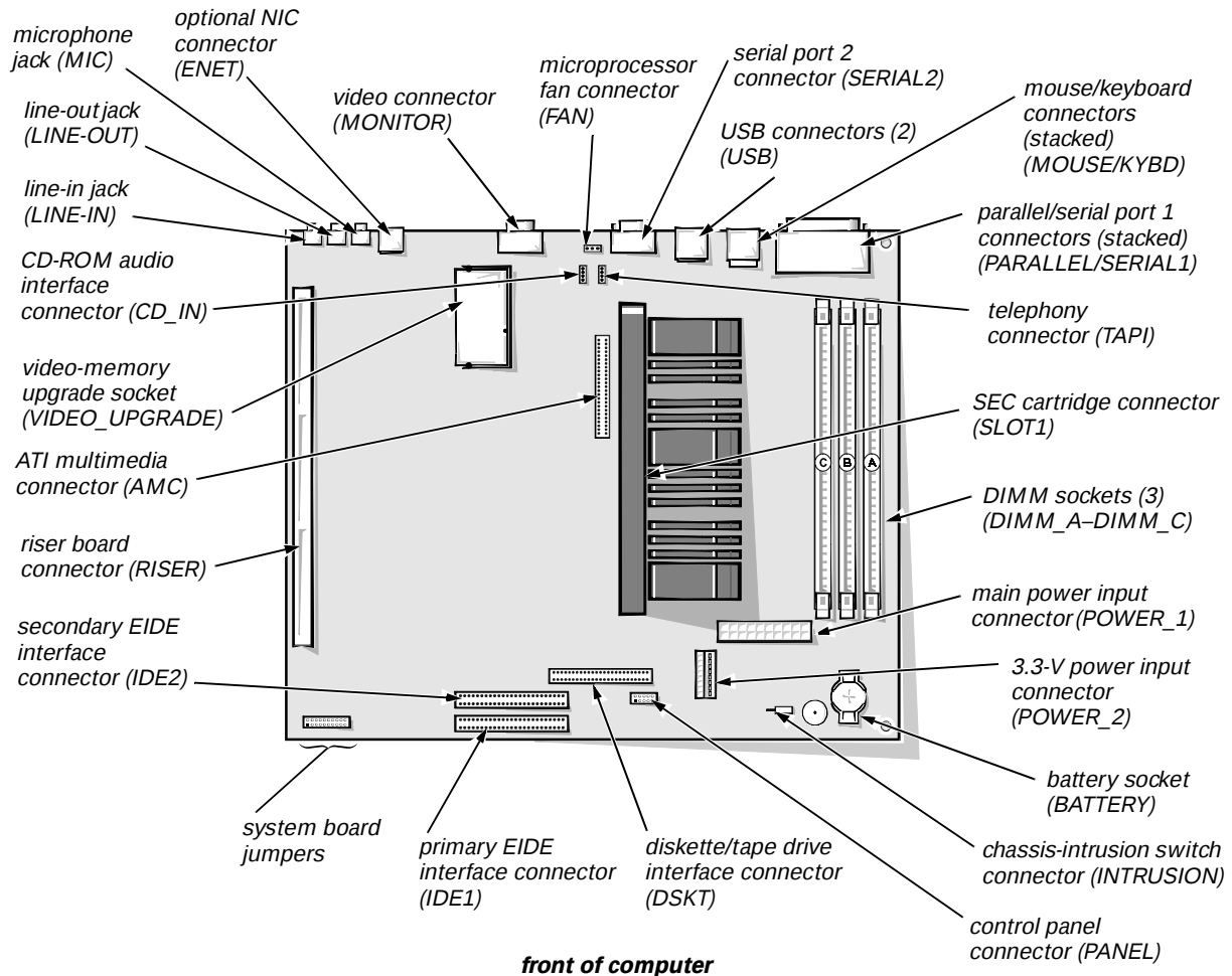
Figure 1-12. System Board Components
