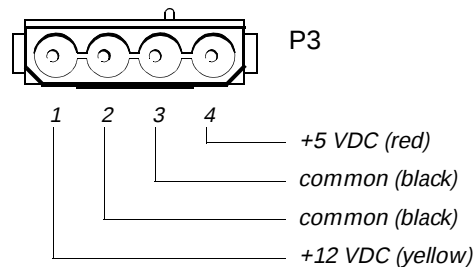
Figure 1-25. DC Power Connector P3 for the OptiPlex NX1 Computer
