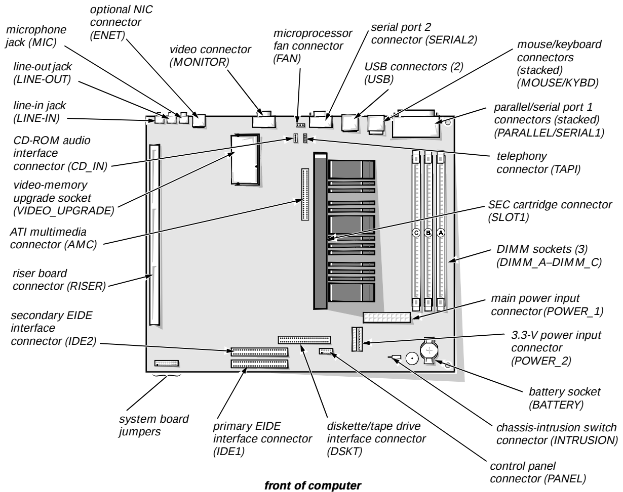
Figure 7-12. System Board Components
