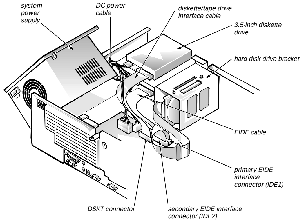
Figure 5-7. Drive Hardware
