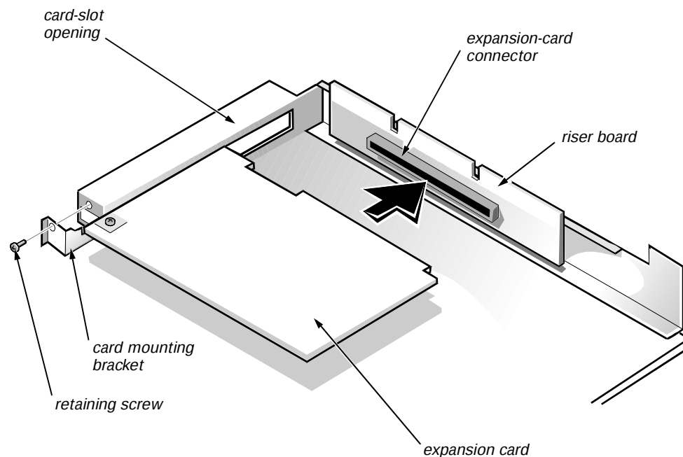
Figure 7-9. Expansion-Card Removal
