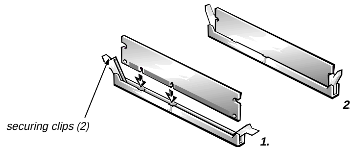
Figure 7-14. DIMM Installation
