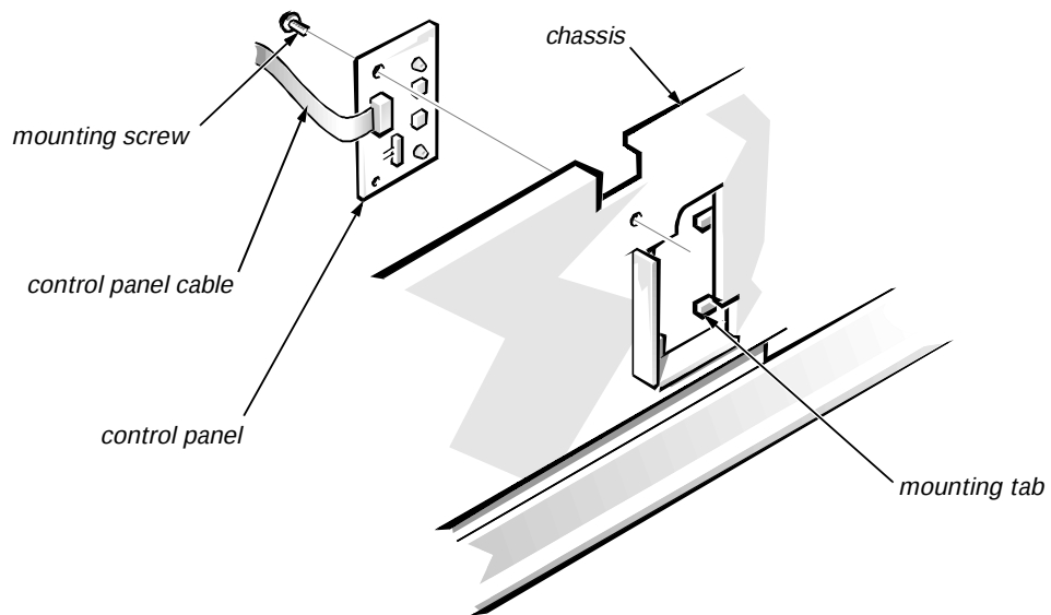
Figure 4-5. Control Panel Removal
