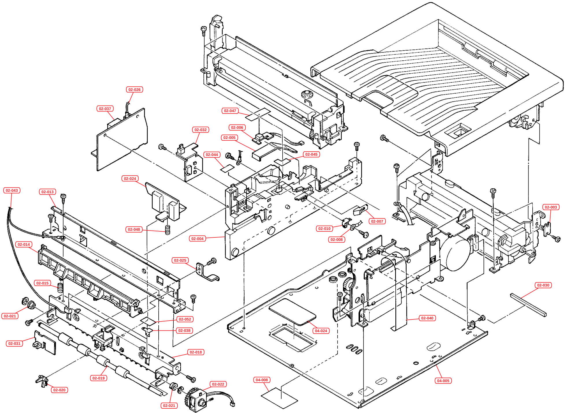
Fig.2 - Frame Unit
