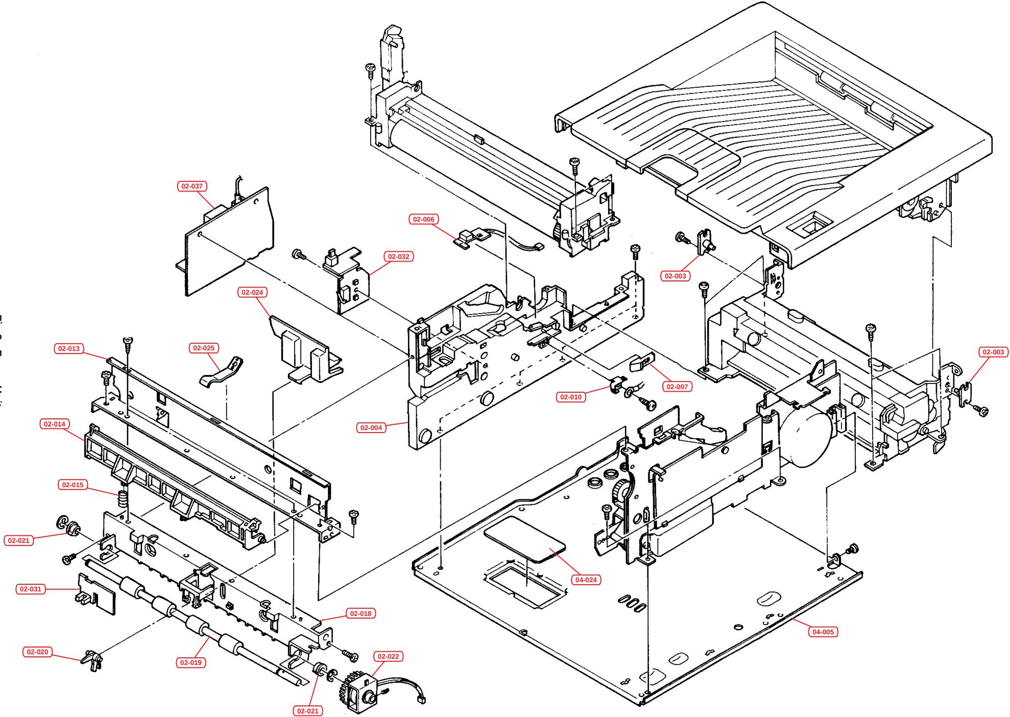
Fig.2 - Frame Unit
