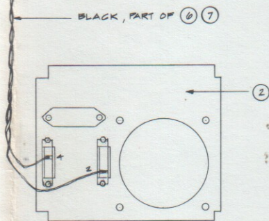
DETAIL A - WIRING
