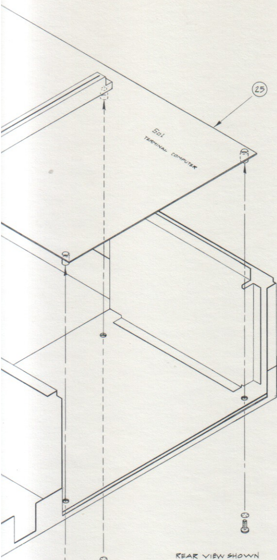
REAR VIEW SHOWN
