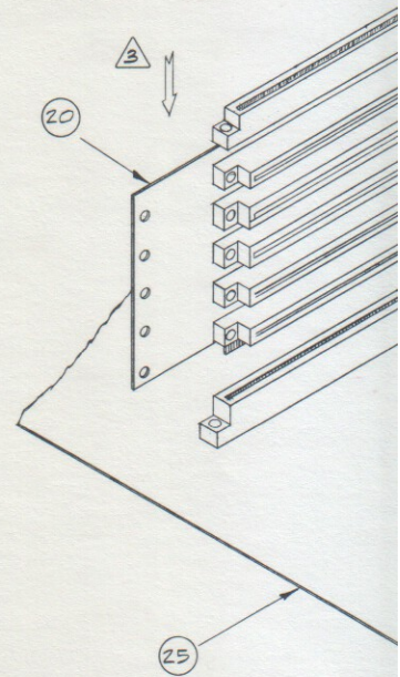
DETAIL - BACKPLANE BOARD
