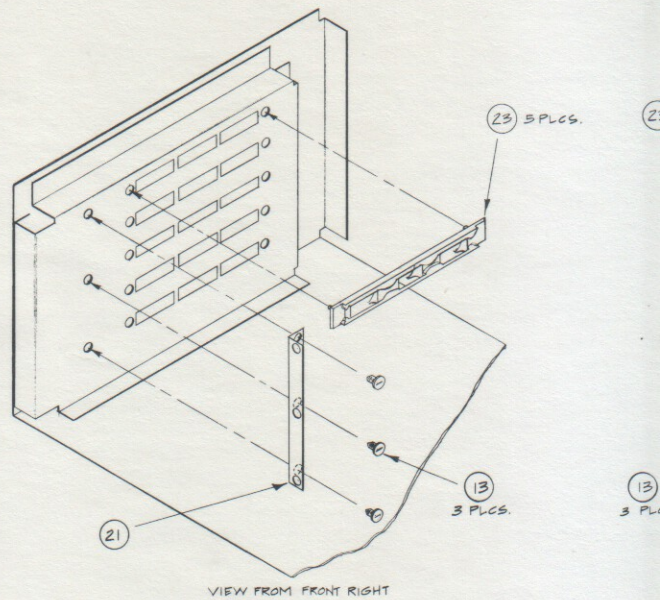
VIEW FROM FRONT RIGHT
