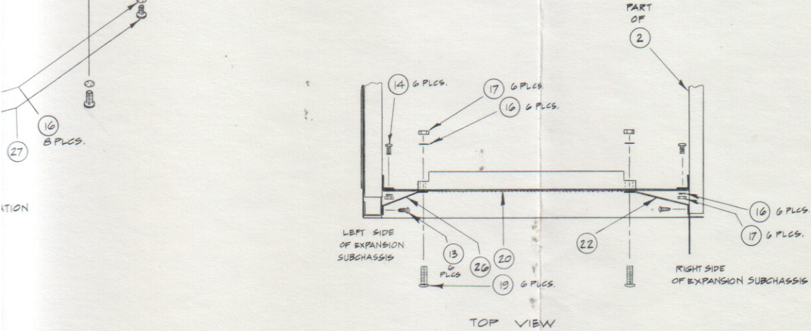
DETAIL - MOUNTING OF BACKPLANE BOARD (Sol-20 ONLY)
