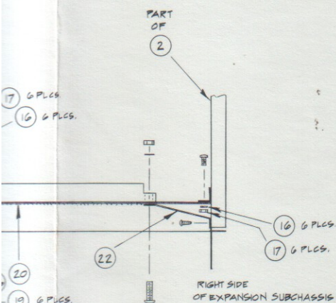
MOUNTING OF BACKPLANE BOARD (S01-20 ONLY)
