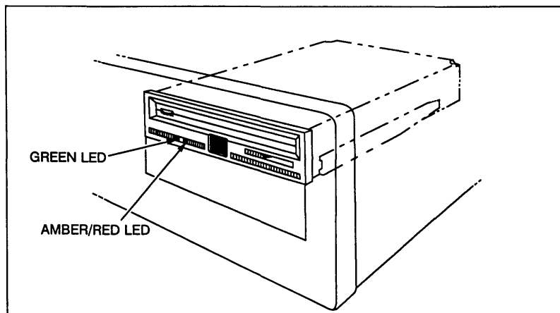
Figure 2-3. The LEDs
