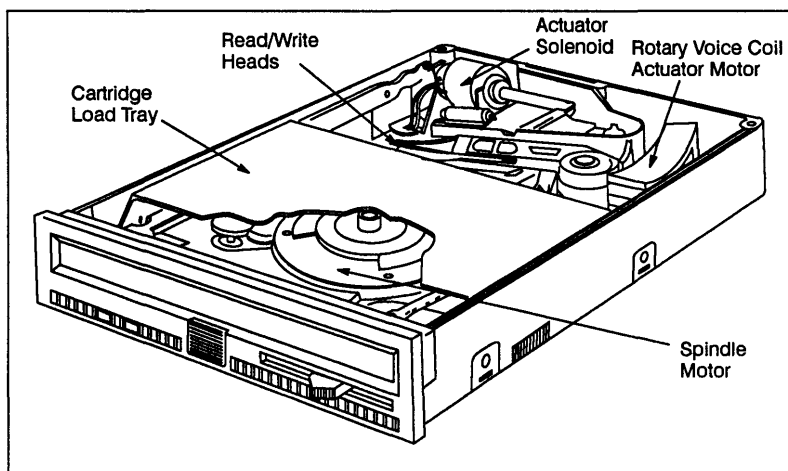
Figure 3-2. Mechanical Components
