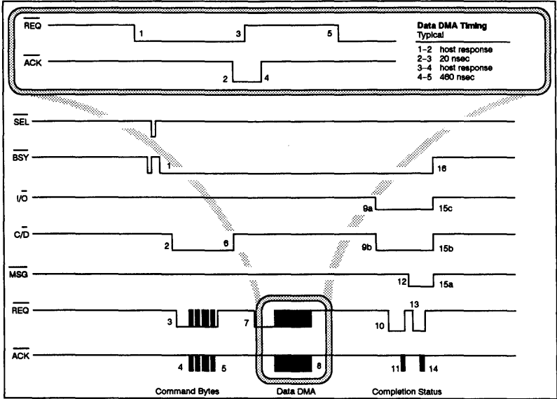
Figure C-2 Write Timing Diagram
