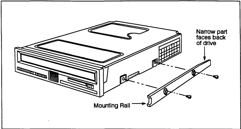
Figure 1-4. Mounting Rails
