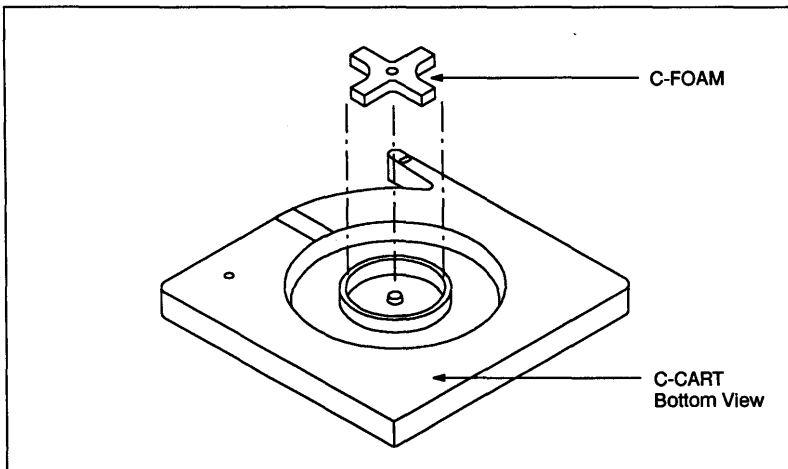
Figure 7-2. C-FOAM Installation
