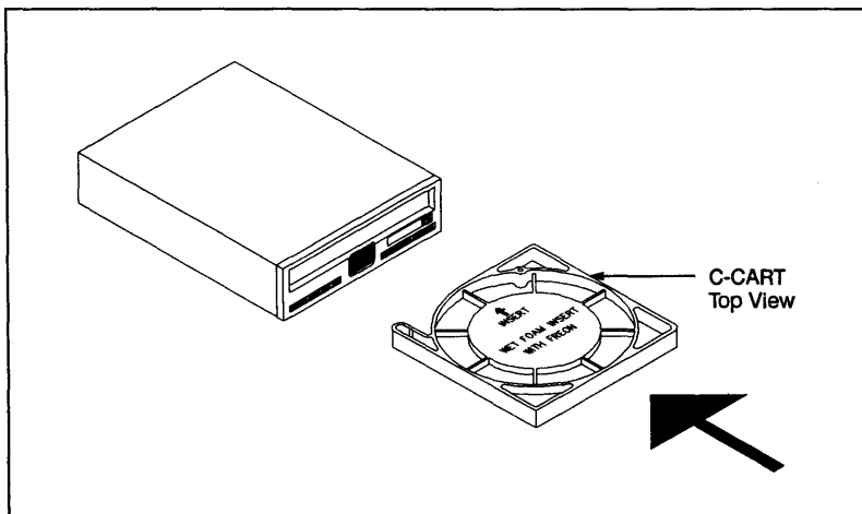
Figure 7-4. C-CART Installation Procedure
