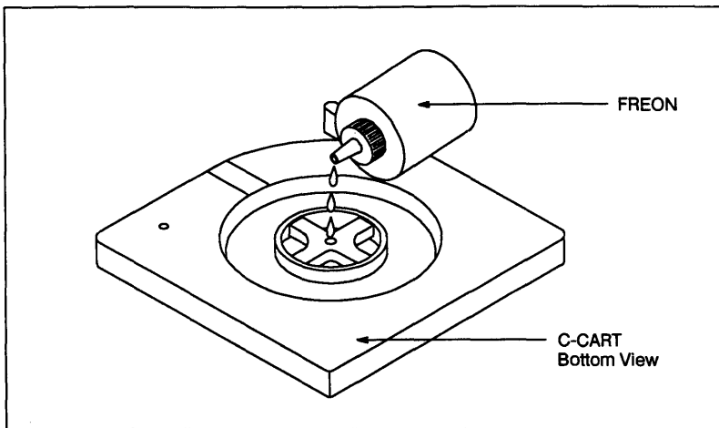
Figure 7-3. Cleaning Fluid Application Procedure
