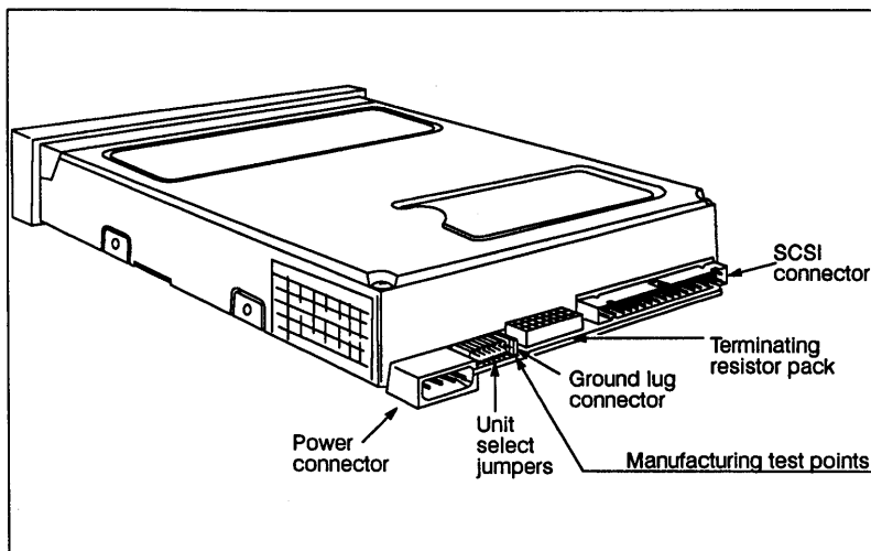
Figure 1-1. SQ555 Physical Interface
