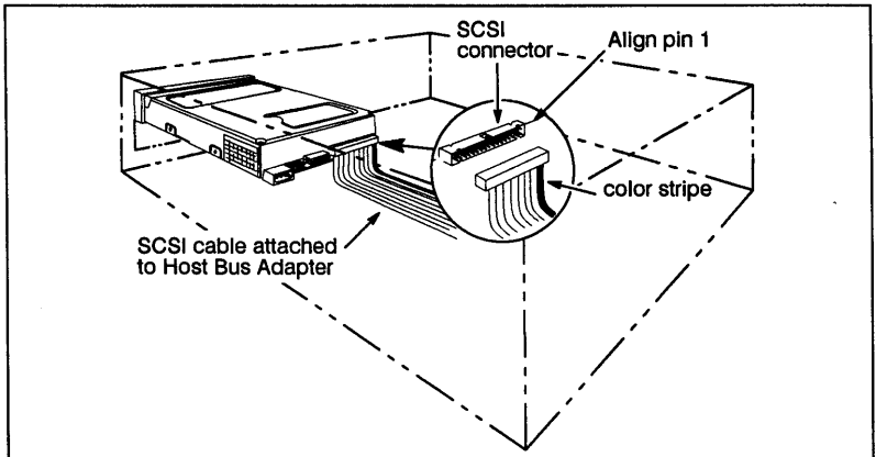
Figure 1-7. Connecting the SCSI Cable
