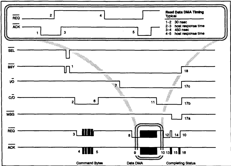
Figure C-1. Read Timing Diagram
