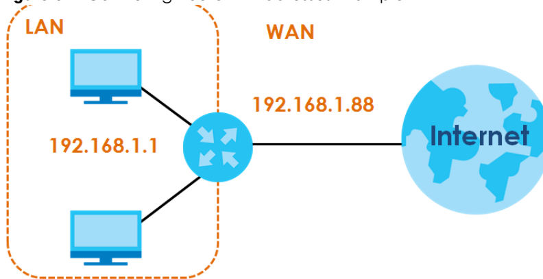
Figure 67 Conflicting Router IP Addresses Example
