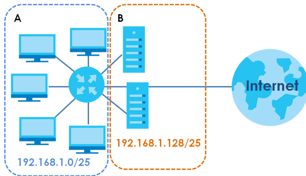
Figure 65 Subnetting Example: After Subnetting
