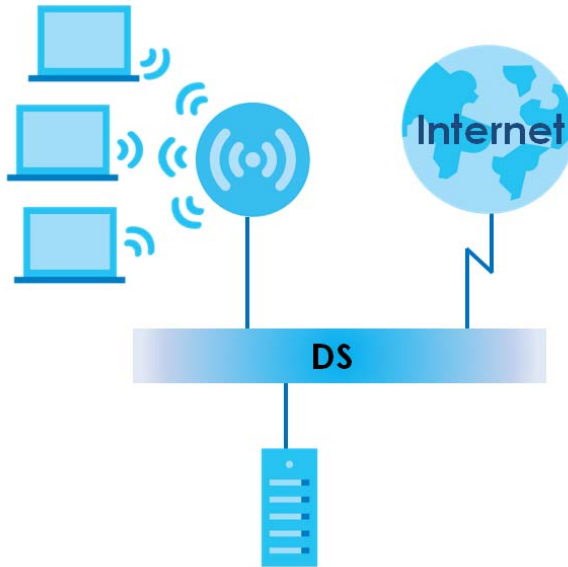
Figure 92 WPA(2) with RADIUS Application Example
