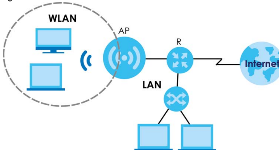
Figure 18 AP Mode
