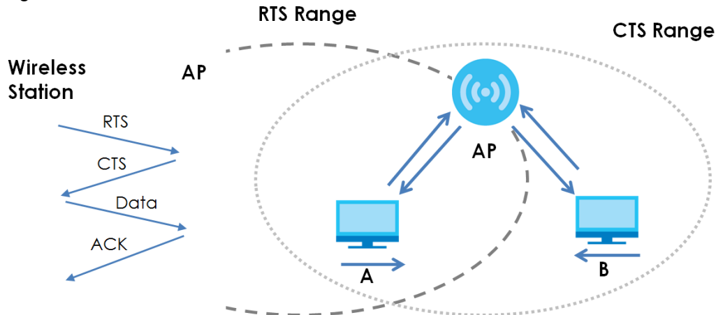
Figure 91 RTS/CTS
